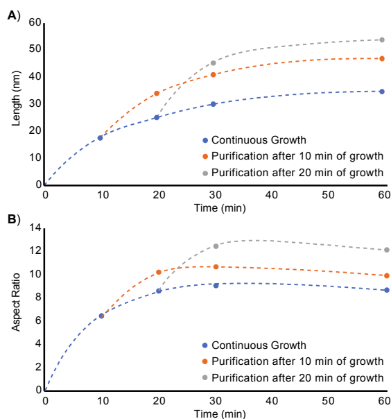
Figure 3. (A) Length and (B) aspect ratio evolution of unseeded CdSe nanorods (blue), nanorods seeded from nanorods grown for 10 minutes (orange), and nanorods seeded from nanorods grown for
