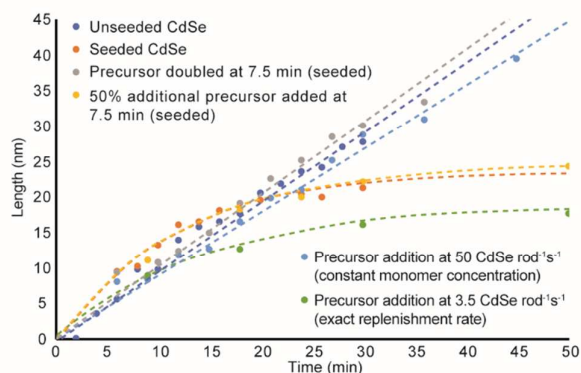
Figure 4. Comparison of length evolution across reaction conditions. For all precursor addition reactions, nanorod growth was seeded by wurtzite CdSe seeds and the precursor addition was initiated at 7.5 minutes.
