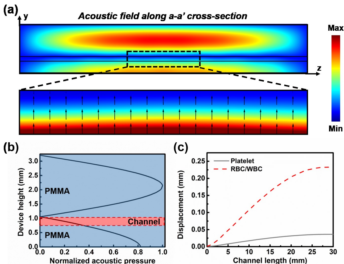
Figure 2. (a) The simulated absolute acoustic pressure field of the a-a' cross-section of the acoustic device for platelet separation, and the Gorkov's potential and acoustic radiation force direction in the channel. (b) The normalized acoustic pressure distribution along the middle line of the acoustic device. (c) The simulated trajectory of the platelets and RBCs/WBCs along the channel length when exposed to the acoustic field.
