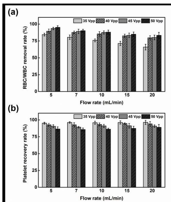
Figure 5. (a) The RBC/WBC removal rate and (b) platelet recovery rate of the acoustic platelet separation device as the functions of the flow rate and driving voltage applied to the acoustic transducer. The data represent three independent experiments as average \pm standard deviation.
