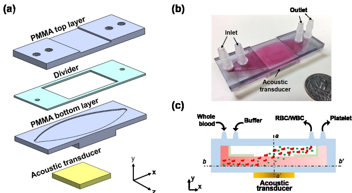
Figure 1. (a) Exploded 3D diagram (an oval channel is also carved into the bottom of the PMMA top layer, which provides a pathway for the buffer solution), (b) photograph, and (c) schematic of the acoustic platelet separation device. a-a' and b-b' are two cross-sections of the device.
