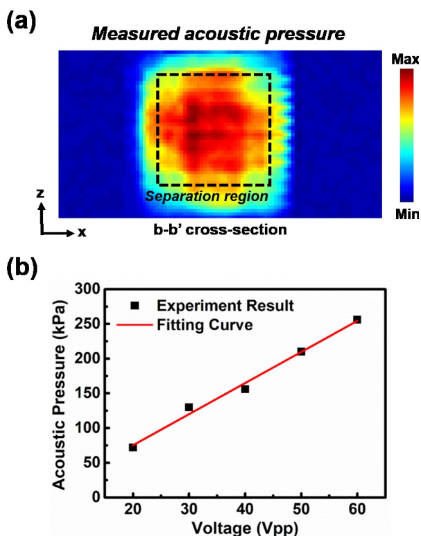
Figure 3. (a) The measured acoustic field of the b-b' cross-section. (b) The measured and fitted acoustic pressure as a function of the driving voltage. Each data point represents five independent measurements \pm standard deviation from a hydrophone; however, because the hydrophone is stable and can reproducibly measure the acoustic pressure, the measured acoustic pressure barely changed among five independent measurements (error bars are smaller than data marker size).
