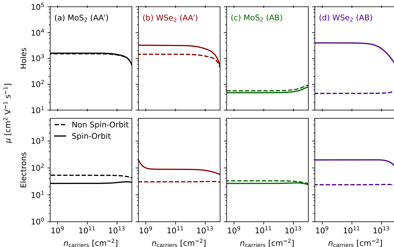
FIG. 3. Calculated mobilities of AA' and AB -stacked transition metal dichalcogenides. In general, the spin-orbit interactions more significantly affect the mobilities in WSe_2 than the MoS_2 , which is a result of its larger predicted splitting and relative energies of valleys at each of the band edges. Both the AA' and AB configurations of WSe_2 show increased mobilities with spin-orbit coupling for the hole and electron cases. Similar to the lifetime in Fig 2, the AB orientation introduces a larger difference between spin-orbit and non spin-orbit predictions than AA' , where there is over an order of magnitude increase for the same reasons described for Fig. 2. Compared to calculated monolayer mobilities, both configurations of the TMDCs have mobilities smaller than their monolayer counterparts, except in the case of the electron mobility of AB -stacked WSe_2 , which is slightly larger in bilayer compared to monolayer when spin-orbit interactions are considered.
