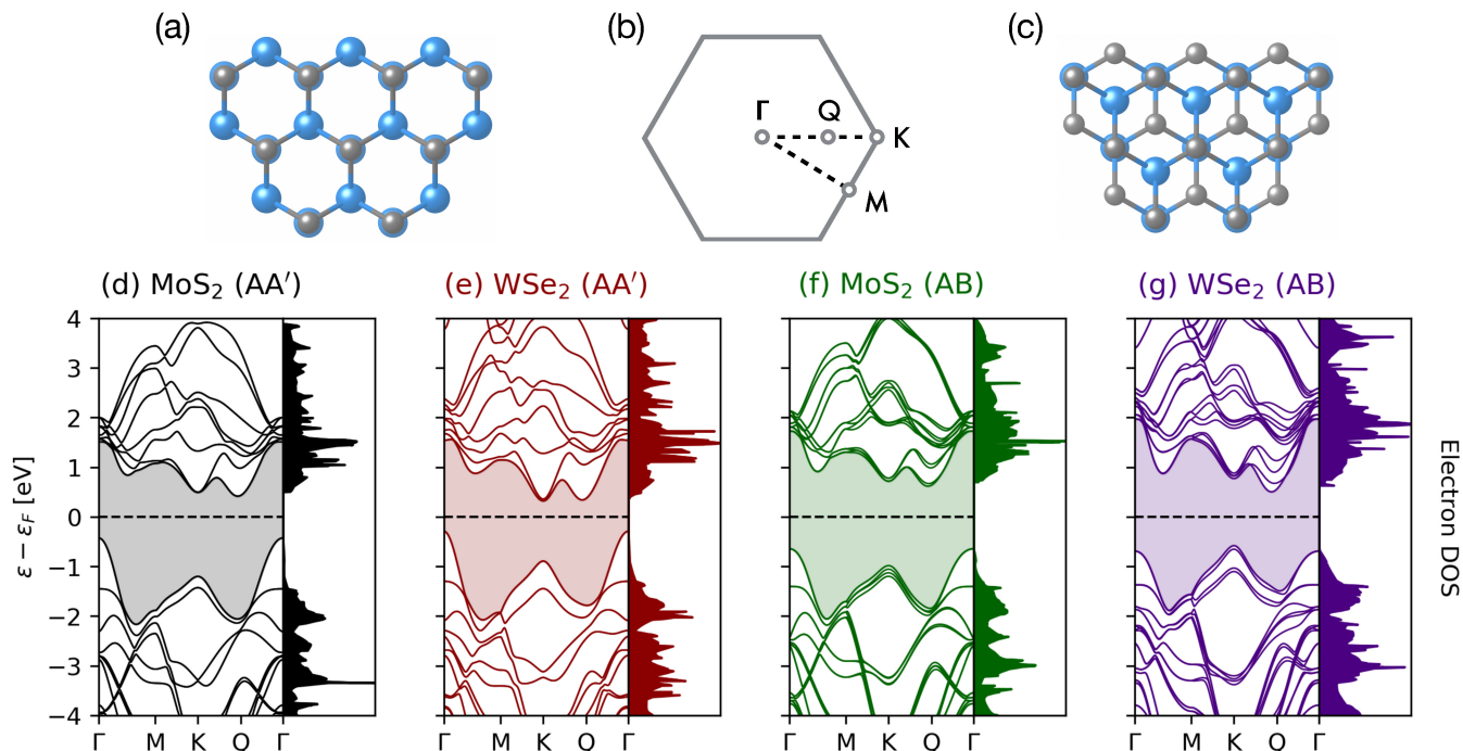
FIG. 1. Bilayer TMDC structure, orientation and electronic structure. Panels (a) and (c) show the stacking arrangement of the two TMDC layers in the out-of-plane direction for the AA' and AB orientation, respectively. The band structures in panels (d)-(g) are plotted along the high-symmetry lines defined by the two dimensional Brillouin zone depicted in panel (b). The conduction band edge states in all cases are at the K and Q points, whereas the valence band edges are at the K and \Gamma points. All four of these points are sensitive to interlayer coupling, and the Q of the conduction band and K of the valence band are split further by a combination of spin-orbit and interlayer coupling. In the AA' orientation, the primary splitting is a result of interlayer coupling, while in the AB orientation, it is the spin-orbit effects which introduce large splitting values. The smaller overall band gap of the AA' orientation is suggestive of stronger interlayer coupling, as the predicted interlayer spacing for these layers is 10% smaller than the spacing in the AB configuration.
