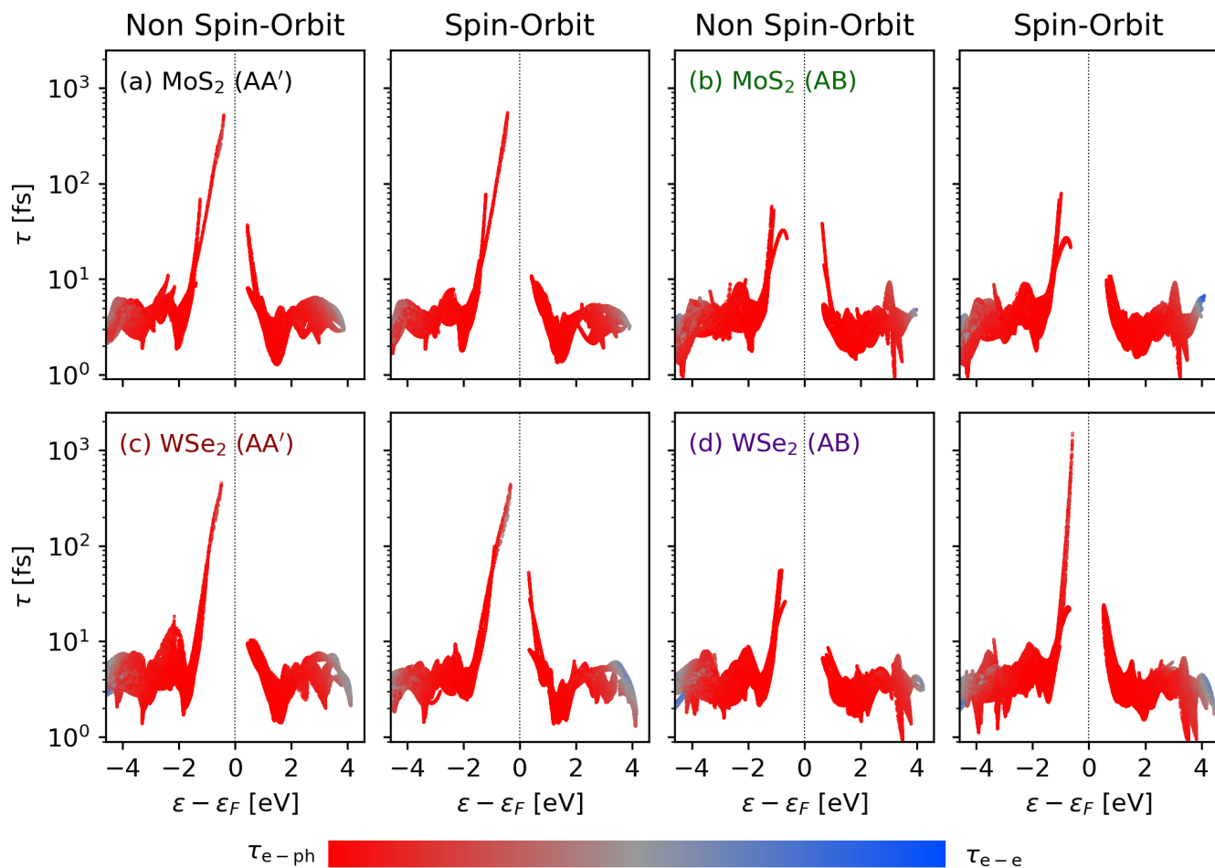
FIG. 2. Calculated scattering lifetimes in each of the bilayer TMDCs studied. The lifetimes in the AA' and AB configurations are relatively similar except at the band edges. The hole lifetimes of both TMDCs are not significantly affected by spin-orbit splitting in the AA' configuration, as the effect of spin-orbit coupling is to increase the already-split valence band edge, which is induced by interlayer coupling. Electron lifetimes are increased in WSe_2 with spin and decreased in MoS_2 with spin because of the relative energies of the Q and K valleys. Spin-orbit coupling pushes the Q point to phonon-accessible energies relative to the K point in MoS_2 , while it pushes the Q valley away from the K valley in the case of WSe_2 . In the AB configuration, hole lifetimes of WSe_2 are found to significantly increase as a result of spin-orbit coupling, while hole lifetimes in MoS_2 are predicted to be relatively unaffected. Similar to the AA' configuration, electron lifetime trends are governed by the relative energies of the Q and K valleys. The relative contribution of electron-electron and electron-phonon interactions to the lifetime is indicated by the colorbar. All scattering observed is dominated by electron-phonon processes.
