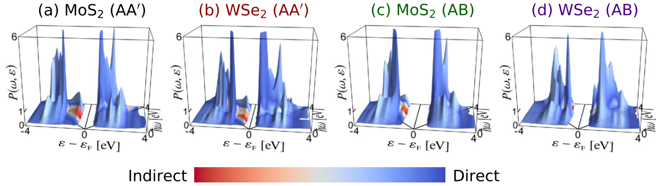
FIG. 4. Hot Carrier generation profiles of AA' and AB-stacked transition metal dichalcogenides. The profiles are normalized and show the likelihood of hot carriers being generated from direct vs. indirect transitions. In all cases, despite the indirect nature of the band gap, transitions are dominated by direct transitions as opposed to indirect. This is an interesting yet surprising result from our calculations. The indirect transitions at the valence band edge suggest that \Gamma valleys can be populated, but their overall density of states limits the quantity of transitions to this energy. Meanwhile, direct transitions associated with the K point dominate the hot carrier generation mechanisms for the photon energy range considered.
