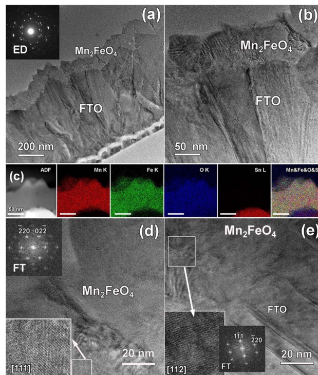
Fig. 8 (a) Cross-sectional low magnification BF-TEM image of a Mn 2 FeO 4 specimen obtained from a Mn:Fe = 2:1 precursor mixture and corresponding ED pattern. (b) Magnified BF-TEM image of Mn 2 FeO 4 /FTO interface. (c) HAADF-STEM image and simultaneously acquired EDXS elemental maps for Mn K, Fe K, O K, Sn L, along with an overlaid color image. (d and e) HRTEM images of Mn 2 FeO 4 grains recorded for two main zone axes, i.e. [111] and [112], respectively. The magnified areas framed by white boxes and corresponding FT patterns are given as insets.
