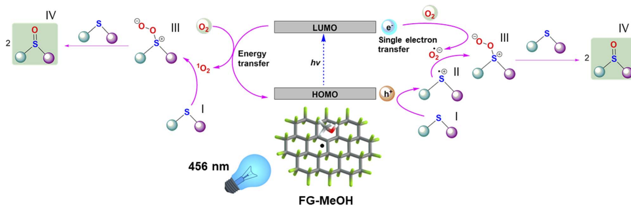
Fig. 3 Proposed mechanisms for the photooxidation of organic sulfides to the corresponding sulfoxides, using FG as a photocatalytic promoter.
