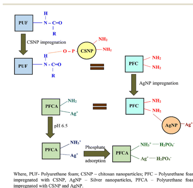
Fig. 5 Schematic illustration of the phosphate adsorption mechanism of PFCA through electrostatic attraction (reprinted with permission from Sasidharan et al. ). 87
