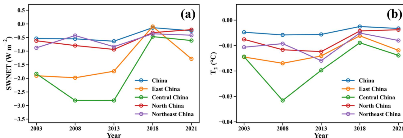
Fig. 3 Regional-mean OCSB-attributable radiative and temperature responses in June for China and its four subregions (East China, Central China, North China, and Northeast China) in 2003, 2008, 2013, 2018, and 2021. (a) Surface net shortwave radiation (SWNET). (b) 2 m air temperature ( T_2 ).
