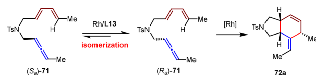
Scheme 19 \text{Rh}(\text{I})/\text{Malphos} -catalyzed dynamic kinetic resolution (DKR) of racemic allene-1,3-dienes via the intramolecular [4+2] cycloaddition.
