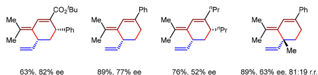
Scheme 21 \text{Pd}(\text{O}) -catalyzed asymmetric intermolecular [4+2] cycloadditions of vinylallenes and 1,3-dienes.
