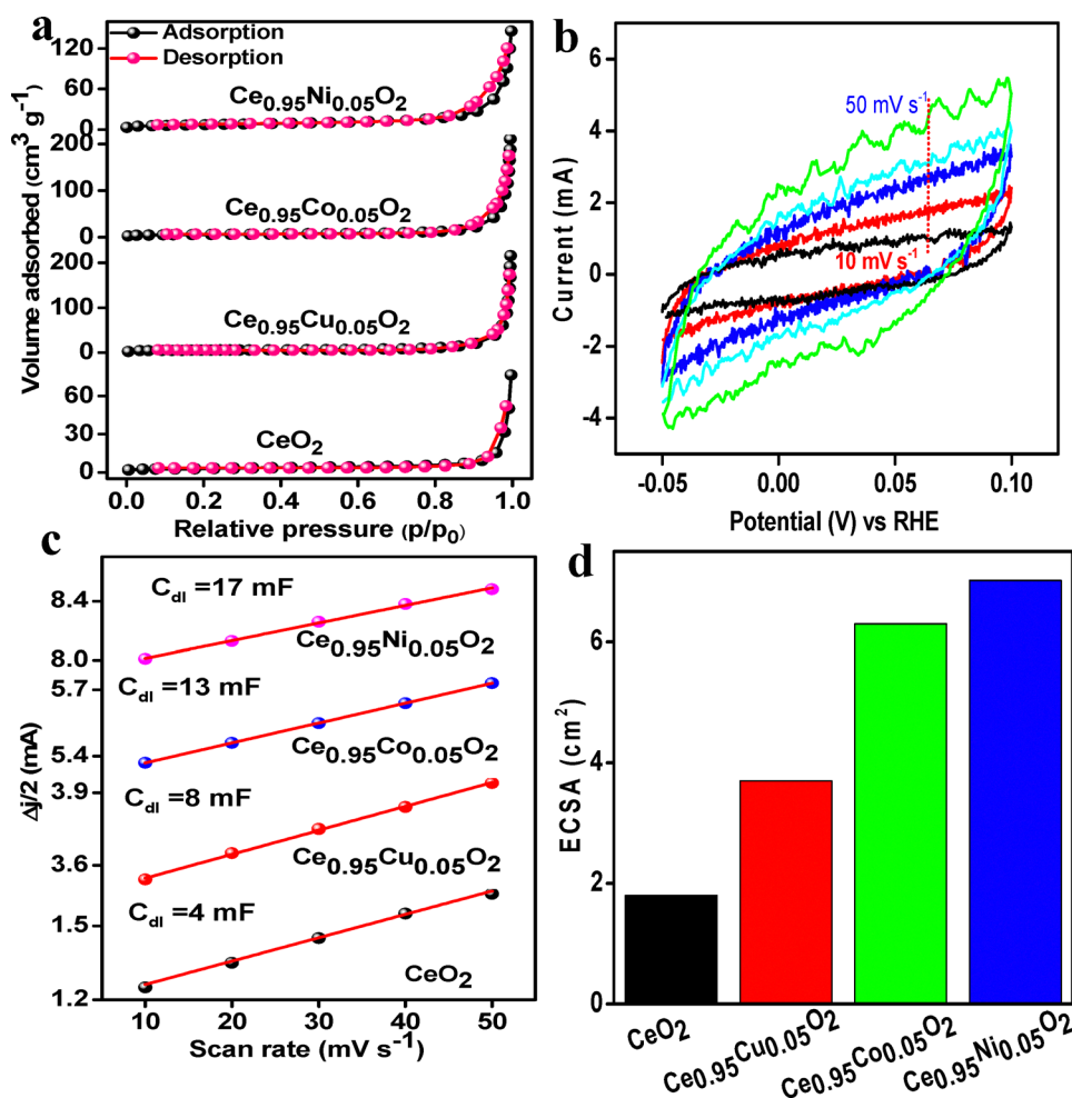
Fig. 3 (a) \text{N}_2 adsorption-desorption isotherms of the synthesized catalysts; (b) CV curves of \text{Ce}_{0.95}\text{Ni}_{0.05}\text{O}_2 in the non-faradaic region ( -0.05 to 0.1 \text{ V} vs. RHE) at scan rates of 10, 20, 30, 40, 50 \text{ mV s}^{-1} ; (c) linear regression between the current density differences in the 0.02 \text{ V} potential window of CV vs. scan rate and (d) ECSA of all four catalysts.
