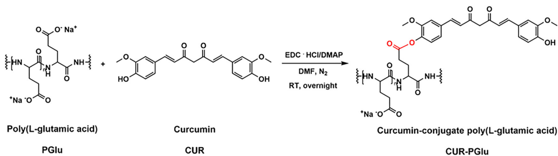
Fig. 2 Scheme of the synthesis of curcumin–conjugate poly(L–glutamic acid) (CUR–PGLu) via an esterification reaction between curcumin (CUR) and poly(L–glutamic acid) (PGLu). The reaction was performed overnight at room temperature (RT) after activating the side chains of PGLu with 1-ethyl-3-(3-dimethylaminopropyl)carbodiimide hydrochloride (EDC-HCl) and dimethylaminopyridine (DMAP).
