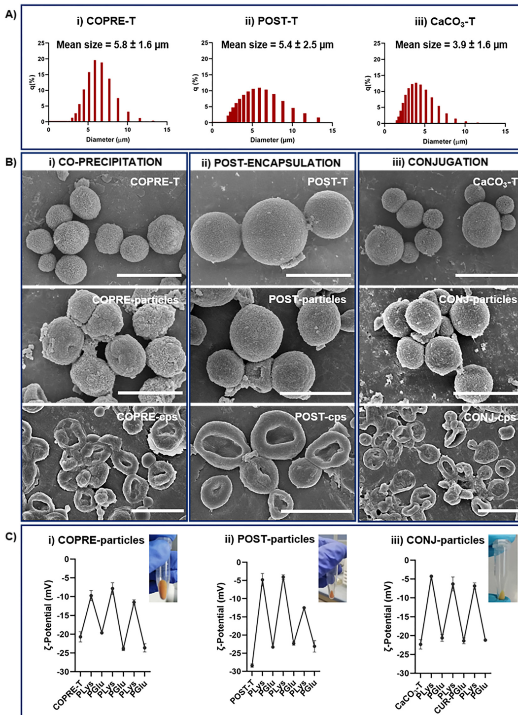
Fig. 4 Characterization of curcumin (CUR)-loaded templates ( i.e. , COPRE-T and POST-T), calcium carbonate template ( \text{CaCO}_3\text{-T} ), and the corresponding layer-by-layer (LbL)-particles and capsules synthesized according to the co-precipitation, post-encapsulation, and conjugation approaches. (A) Size distribution of COPRE-T (i), POST-T (ii), and \text{CaCO}_3\text{-T} (iii), respectively. (B) Micrographs of the templates, LbL-particles, and LbL-capsules (from top to bottom) obtained for each formulation. The scale bar is 5 \mu\text{m} . (C) \zeta -potential values measured during the LbL process after the deposition of each polypeptide layer in COPRE-particles (i), POST-particles (ii), and CONJ-particles (iii). Insets show photographs of the LbL-particles, highlighting the yellowish color associated with the presence of CUR. The values are reported as mean \pm standard deviation (SD); N = 3 .
