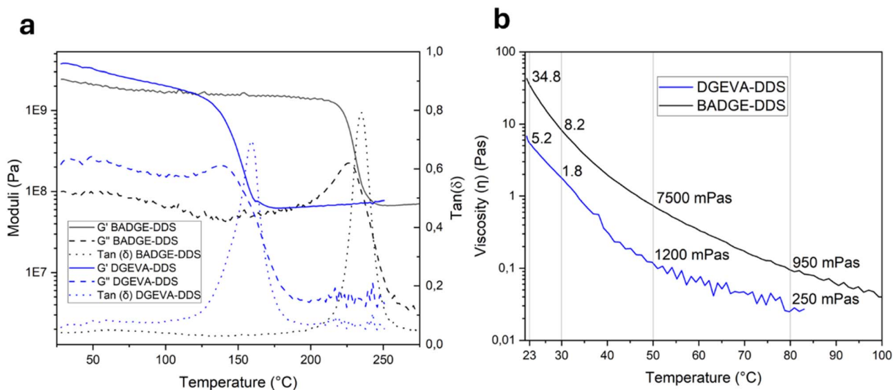
Fig. 2 (a) DMA temperature sweep in the three point bending setup of both systems. Heating rate = 1 K \text{min}^{-1} . (b) Viscosity vs. temperature profiles of both systems.
