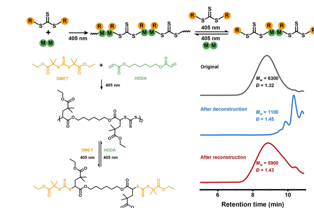
Fig. 1 Deconstruction and repolymerization of RAFT step-growth polymer prepared with [DMET]_0 : [HDDA]_0 = 1 : 1 for 12 hours under irradiation of a 405 nm LED.
