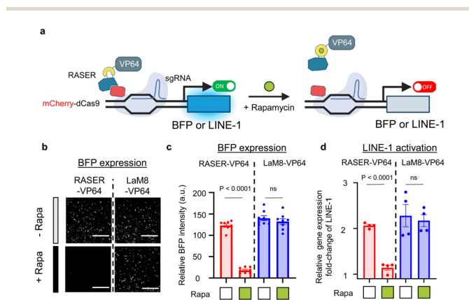
Fig. 4 RASER applied to achieve rapamycin-induced shutdown of customized gene expression. Data are presented as mean \pm sem. (a) Cartoon illustrating the design of a rapamycin-switchable split CRISPRa system made of mCherry-dCas9 and RASER-VP64. In the absence of rapamycin, RASER-VP64 interacts with mCh-dCas9 to induce gene expression. Upon rapamycin treatment, RASER-VP64 dissociates from mCh-dCas9 to terminate transcriptional activation. BFP is used as a reporter for dCas9-VP64-mediated transcriptional regulation. (b) Confocal images showing BFP expression in HeLa cells transfected with the rapamycin-activatable CRISPRa system (RASER-VP64 + mCh-dCas9) or the positive control vectors (LaM8-VP64 + mCh-dCas9) before and after overnight rapamycin treatment. Scale bar, 500 \mu m. (c) Quantification of BFP signals before and after rapamycin treatment (as shown in panel b). n = 8 fields of view from three independent assays. (d) Bar graph showing the relative human LINE-1 expression in HEK293T cells, measured by real-time RT-PCR, for cells coexpressing the indicated constructs with specific guide RNAs, compared to the control group with non-targeting guide RNAs. ns, not statistically significant.
