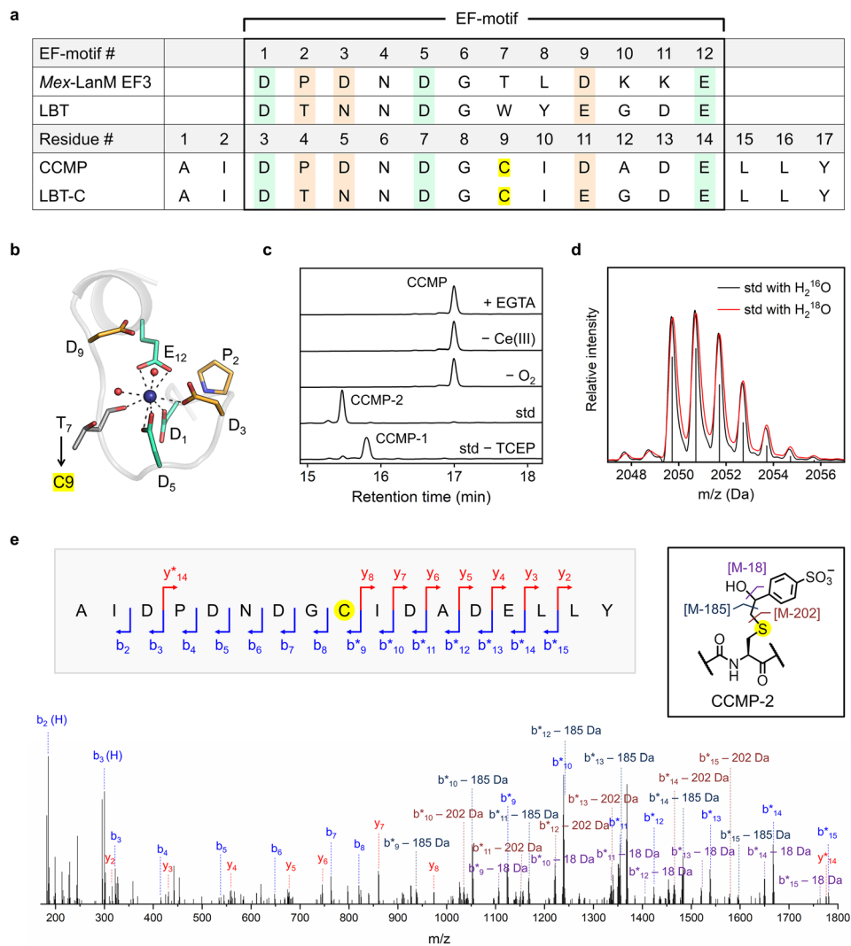
Fig. 2 Design of Ce(III)-binding peptides for site-specific oxidative thiol–ene coupling. (a) Amino acid sequences of Mex-LanM EF3, LBT, and CCMP mutants. EF-hand motifs are highlighted by a bold-bordered box. (b) A previously reported X-ray crystal structure of the 3rd EF-hand of Mex-LanM (PDB code: 8fns). Metal (Nd(III)) and metal-bound water molecules are shown with blue and red spheres, respectively. (c) HPLC analysis of the reactions with 100 \mu M Ce(III)(CCMP) and 10 mM 4VBS in 50 mM Tris–HCl, pH 7.4, followed by 1 mM TCEP treatment and the modified conditions. (d) Negative-ion mode MALDI-TOF/TOF analysis of CCMP-2 from the reactions with \text{H}_2^{16}\text{O} or \text{H}_2^{18}\text{O} . Vertical drop lines indicate the calculated isotope mass distribution of CCMP-2 [\text{M}-\text{H}]^- . (e) Tandem mass spectrometry fragmentation analysis of CCMP-2. Asterisks indicate the peptide fragments containing the modified cysteine.
