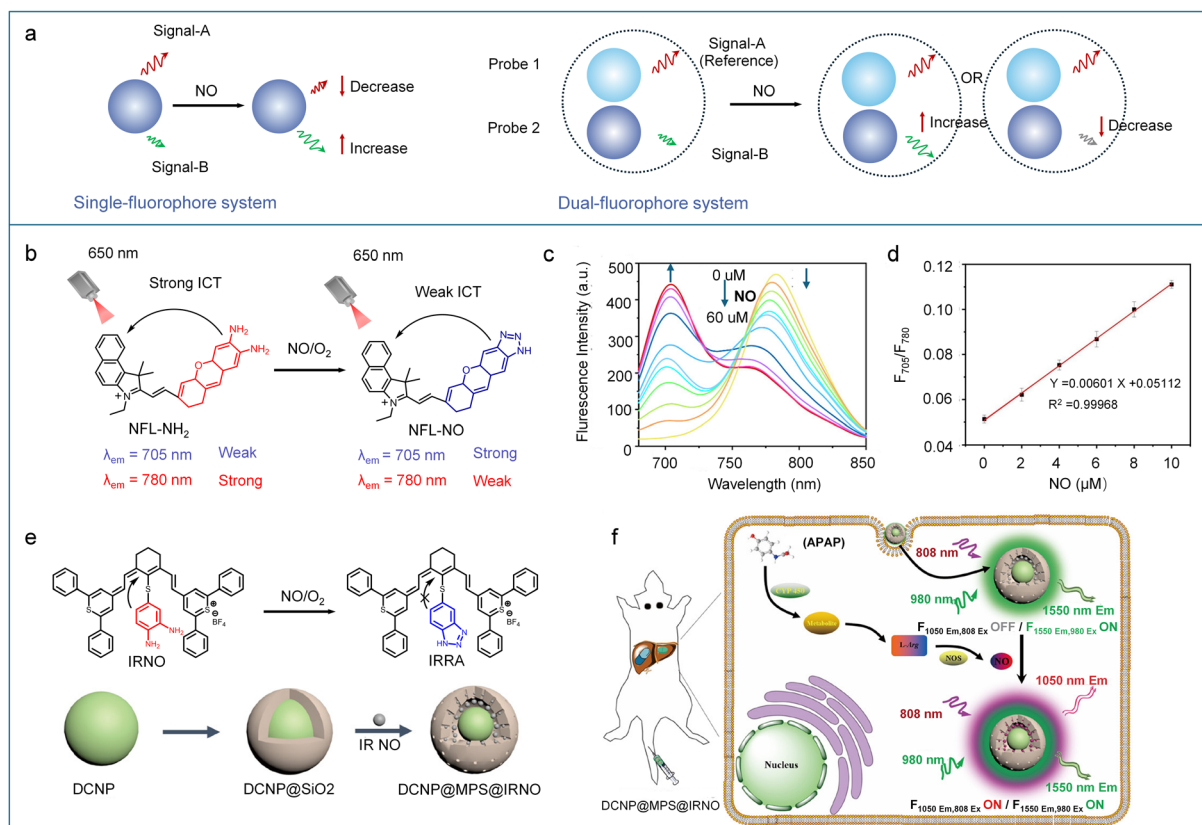
Fig. 5 (a) The general strategies for constructing NO-responsive ratiometric fluorescent probes. (b) Ratiometric probe NFL-NH 2 . (c) Fluorescence intensity of NFL-NH 2 after adding the NO donor (0–60 \mu\text{M} ) in ethanol solution. (d) Linear relationship between fluorescence intensity ratio ( F_{705}/F_{780} ) and NO concentration (0–10 \mu\text{M} ). Reproduced from ref. 32 with permission from American Chemical Society, copyright 2024. (e) The response mechanism of IRNO toward NO and the preparation of the NO-responsive nanoprobe DCNP@MPS@IRNO. (f) Illustration of the NO-responsive nanoprobe DCNP@MPS@IRNO for in vivo monitoring of liver injury induced by drug overdose. Reproduced from ref. 82 with permission from American Chemical Society, copyright 2021.
