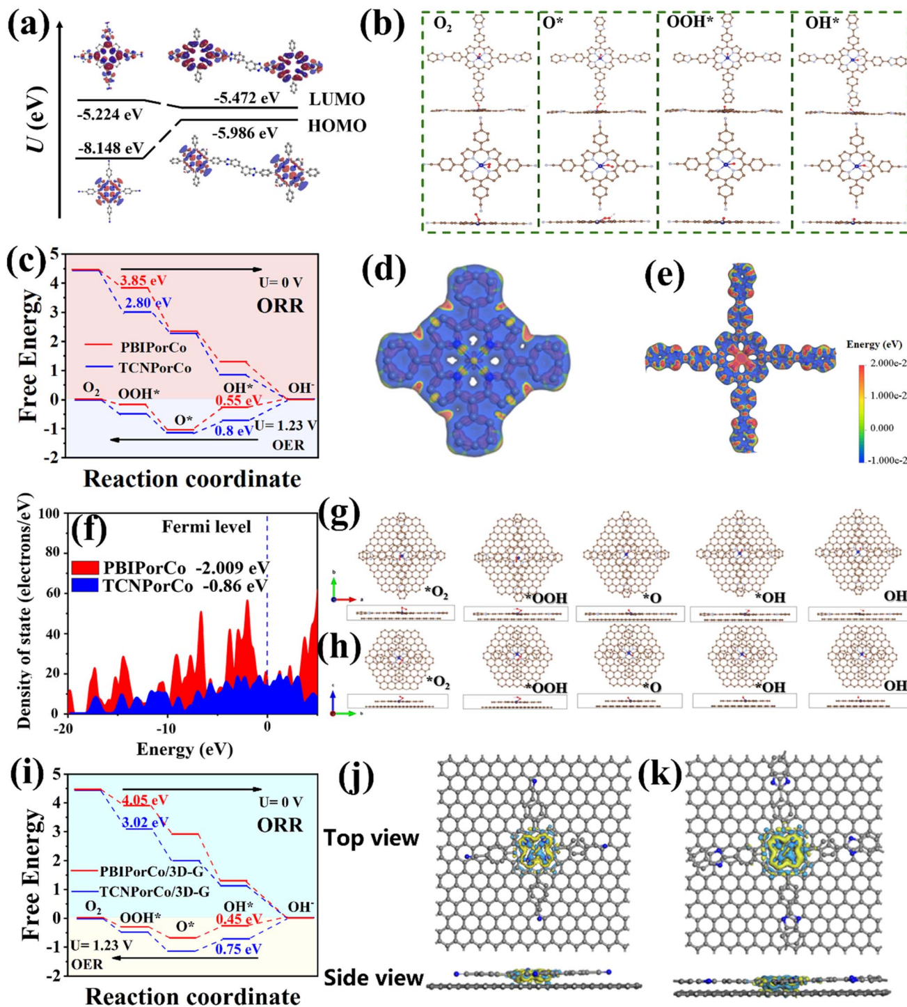
Fig. 6 DFT calculations. (a) The energy levels of the HOMO and LUMO of TCNPorCo and PBIPorCo; (b) PBIPorCo and TCNPorCo adsorption intermediate models ( \text{Co-N}_4 site); (c) Gibbs free energy change ( \Delta G ) of TCNPorCo and PBIPorCo after ORR and OER; (d and e) electrostatic potential (ESP) of TCNPorCo and PBIPorCo; (f) DOS of TCNPorCo and PBIPorCo; (g and h) adsorption oxygen intermediate models for the PBIPorCo/3D-G and PorCo/3D-G repeating unit ( \text{Co-N}_4 site); (i) Gibbs free energy change ( \Delta G ) of TCNPorCo and PBIPorCo after ORR and OER; (j and k) charge density difference of PBIPorCo/3D-G and PorCo/3D-G.
