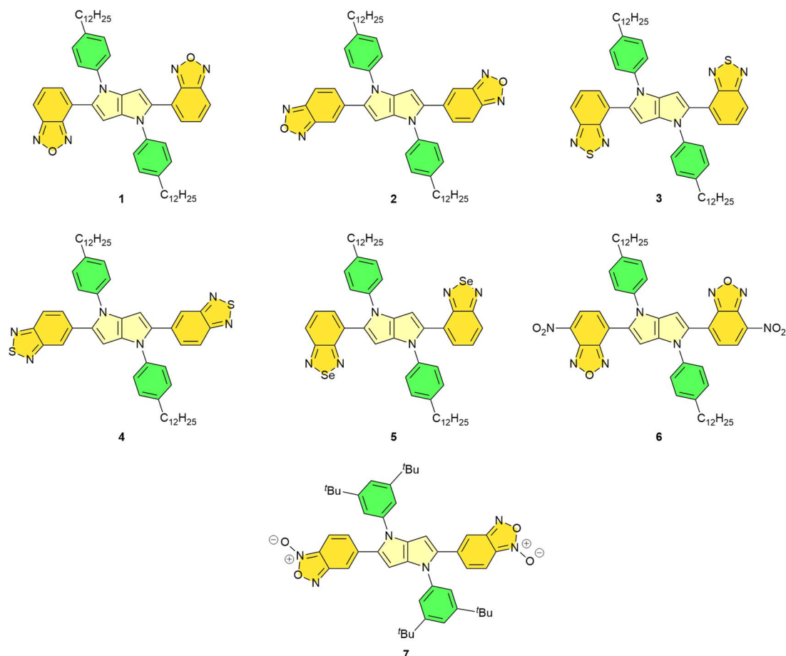
Fig. 1 Structures of quadrupolar tetraarylpyrrolo[3,2- b ]pyrroles 1–7.
