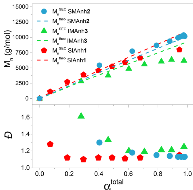
Fig. 2 Evolution of M_n^{\text{SEC}} and D with increasing monomer conversion for well-controlled SMAAnh, SIAnh and IMAAnh copolymerizations.
