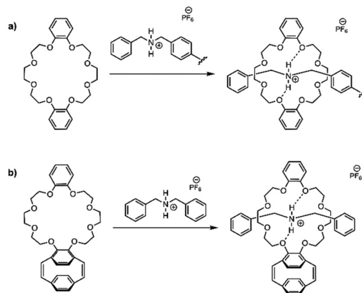
Scheme 6 Pseudorotaxane formation. (a) The host is commercially available DB24C8 and the guest is PS-DBA + , 22 . (b) The host is CE- p Cpd, 10 , and the guest is commercially available DBA + .
