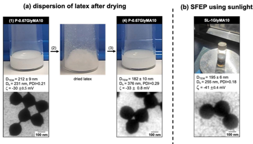
Fig. 6 Sustainability of photo-SFEP process. (a) (1) Surfactant-free latex prepared via photo-SFEP of GlyMA under 405 nm irradiation using R = 0.67\% at SC = 10 \text{ w/w} . (2) The nanoparticles were lyophilized and subsequently (3) re-dispersed in water targeting initial SC = 10 \text{ w/w} . (b) Surfactant-free latex prepared via photo-SFEP of GlyMA under sunlight using R = 1\% at SC = 10 \text{ w/w} in water.
