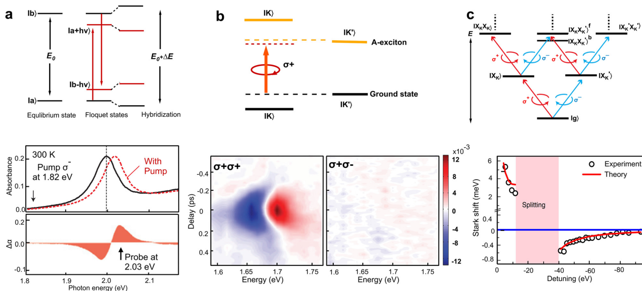
Fig. 7 (a) Upper panel: energy level diagram of two-level |a\rangle and |b\rangle atoms showing that the equilibrium and photo-dressed state |a + \hbar\nu\rangle and |b - \hbar\nu\rangle , resulting in energy shifted after hybridization via optical Stark effect in WS 2 . Lower panel: measured absorbance of monolayer WS 2 (black) and a hypothetical absorbance curve (dashed) that simulates the optical Stark effect. Reproduced with permission from ref. 128. Copyright 2014, Springer Nature Limited. (b) Upper panel: schematic of the optical Stark effect in WSe 2 for valley transitions with nonresonant, left circularly polarized \sigma^+ pump. The dashed black and yellow lines denote the unperturbed ground and exciton states, respectively. Lower panel: transient reflection spectra of A-exciton resonance at 77 K. with probe helicity same and opposite from pump, respectively. Reproduced with permission from ref. 131. Copyright 2014, Springer Nature Limited. (c) Upper panel: an illustration of optical transition and selection rules for excitons and many-body biexciton states. |g\rangle , |X_K\rangle ( |X_{K'}\rangle ) and |X_K X_K\rangle ( |X_K X_{K'}\rangle ) denote the ground state, K ( K' ) valley exciton state and intra-/inter-valley biexciton states. Lower panel: optical Stark shift of the K' -valley exciton is well defined away from the exciton–biexciton resonance, and it changes from a redshift at large |\Omega_X| to a blueshift at small |\Omega_X| . The experimental data (black circles) agree quantitatively with the prediction of the theoretical model (red lines). Reproduced with permission from ref. 132. Copyright 2018, Springer Nature Limited.
