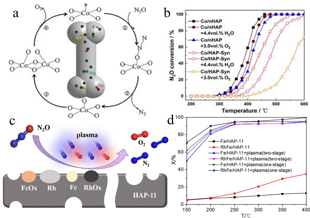
Fig. 6 (a) Break down of N_2O over the surface of Co-doped bone-derived hydroxyapatite (Co/nHAP) catalysts. (b) N_2O decomposition profile. 62 Reproduced with permission from Elsevier (Copyright©2020). (c) Mechanism of plasma-assisted N_2O degradation over the surface of bimetallic RhFe/HAP catalysts. (d) Variation in % N_2O decomposition w.r.t. temperature on RhFe/HAP and Fe/HAP catalysts. 87 Reproduced with permission from Springer-Nature (Copyright©2023).
