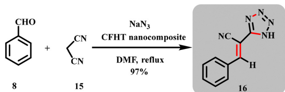
Scheme 7 Catalytic synthesis of 5-substituted 1 H -tetrazole derivatives (Hajjzadeh et al. ).
