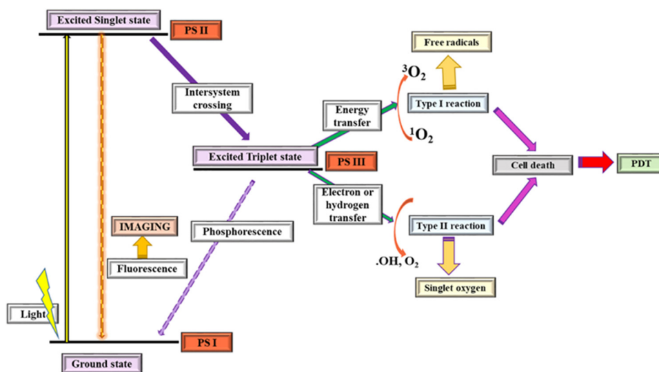
Fig. 1 Photodynamic reaction process (reproduced with permission from ref. 21. Copyright 2019, Elsevier).
