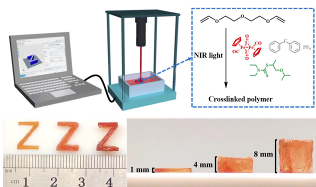
Fig. 6 RAFT stereolithography process under NIR light at 25 °C used to 3D print objects with different thicknesses. Reproduced with permission. Copyright 2021 American Chemical Society. 85
