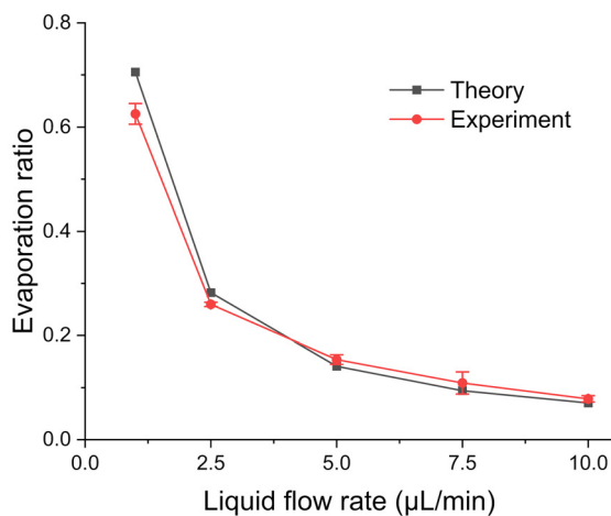
Fig. 6 Deionized water evaporation and corresponding concentration factors under experimental conditions of 30 °C temperature and a 50 mL min -1 dry nitrogen gas flow rate. (a) Evaporation ratio versus liquid flow rate from 1 to 10 μL min -1 . (b) Concentration factor versus liquid flow rate from 1 to 10 μL min -1 .
