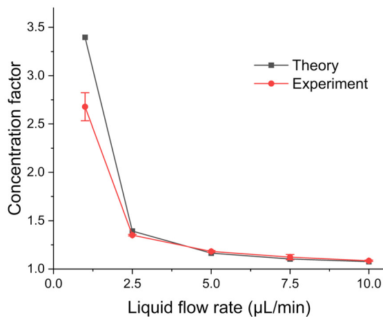
Fig. 6 Deionized water evaporation and corresponding concentration factors under experimental conditions of 30 °C temperature and a 50 mL min -1 dry nitrogen gas flow rate. (a) Evaporation ratio versus liquid flow rate from 1 to 10 μL min -1 . (b) Concentration factor versus liquid flow rate from 1 to 10 μL min -1 .
