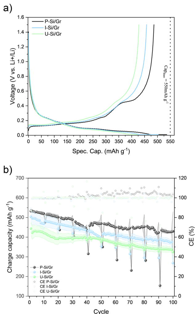
Fig. 6 (a) Voltage profile of the third cycle at C/10. (b) Cycling performance (solid lines, left axis) and coulombic efficiency (CE, hollow circle, right axis) of pristine (P-Si/Gr), and recycled (I-Si/Gr and U-Si/Gr) half-cells over 100 cycles at different C-rates.
