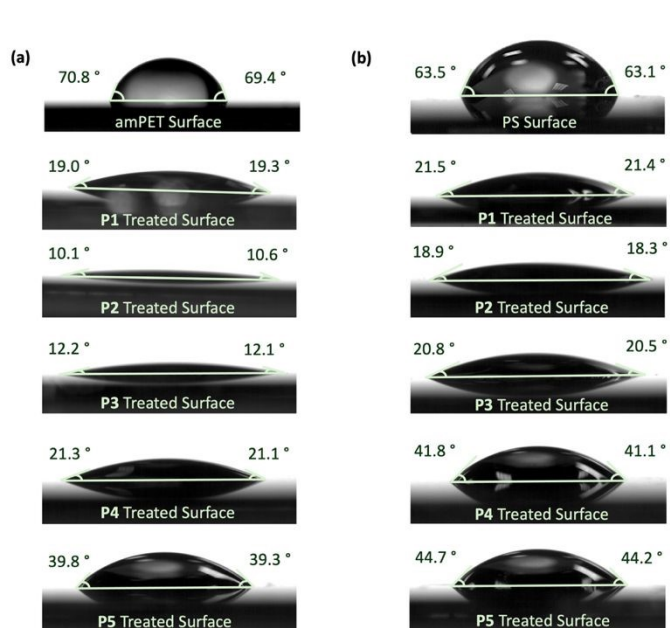
Figure 6: Contact angle measurements of a 5 µL droplet of deionised water on a (a) amPET surface and 1% (w/w) SRP-treated amPET surface; (b) PS surface and 1% (w/w) SRP-treated PS surface; after dip rinsing in H 2 O.
