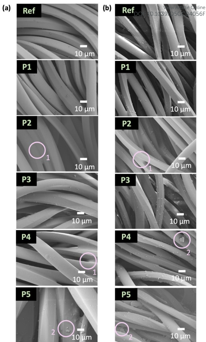
Figure 7: SEM images taken at a magnification of 1,000 × for (a) PET and the PE-SRP modified fabrics ( P1 to P5 ) with a gold-palladium sputter coating thickness of around 33 nm; (b) PS and the PS-SRP modified fabrics ( P1 to P5 ) with a gold-palladium sputter coating thickness of around 49 nm. Some features have been highlighted: 1. SRPs appearing to deposit between fibres; 2. Irregular deposits on fibres.
