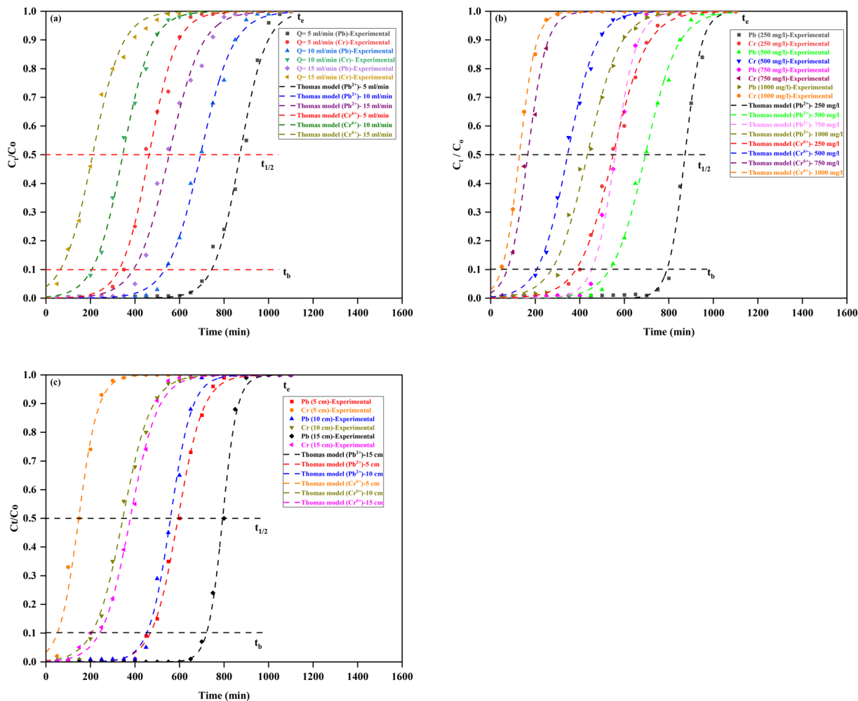
Fig. 20 Thomas model fittings for the column studies to remove Pb 2+ and Cr 6+ : (a) change in the flow rate; (b) change in metal concentration; (c) change in the bed height.
