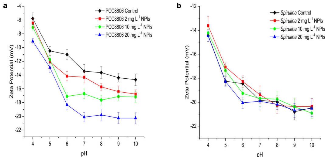
Fig. 3 Surface charge of PCC8806 and Spirulina under PS NPI exposure. Effects of PS NPIs on the ZPs of a. PCC8806 and b. Spirulina cells at the exponential phase in 0.1 M \text{NaNO}_3 at pH 4–10. Values are shown as mean \pm SD, n = 15 . Statistical significance is defined as p < 0.05 .
