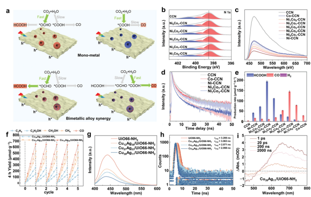
Fig. 5 (a) Schematic diagram of the reaction mechanism of photoreduction of CO 2 by the Ni x Cy-CCN catalyst. (b) XPS spectra of N 1s, (c) PL spectra and (d) time-resolved transient PL decay spectra for Ni x Cy-CCN. (e) Product evolution rates of Ni x Cy-CCN. Reproduced with permission from ref. 50. Copyright 2024, Wiley-VCH. (f) The cycling test over Cu x Ag 50-x /UiO66-NH 2 . (g) PL spectra; (h) time-resolved transient PL decay spectra and (i) Fs-TA spectra of Cu x Ag 50-x /UiO66-NH 2 . Reproduced with permission from ref. 51. Copyright 2024, Royal Society of Chemistry.
