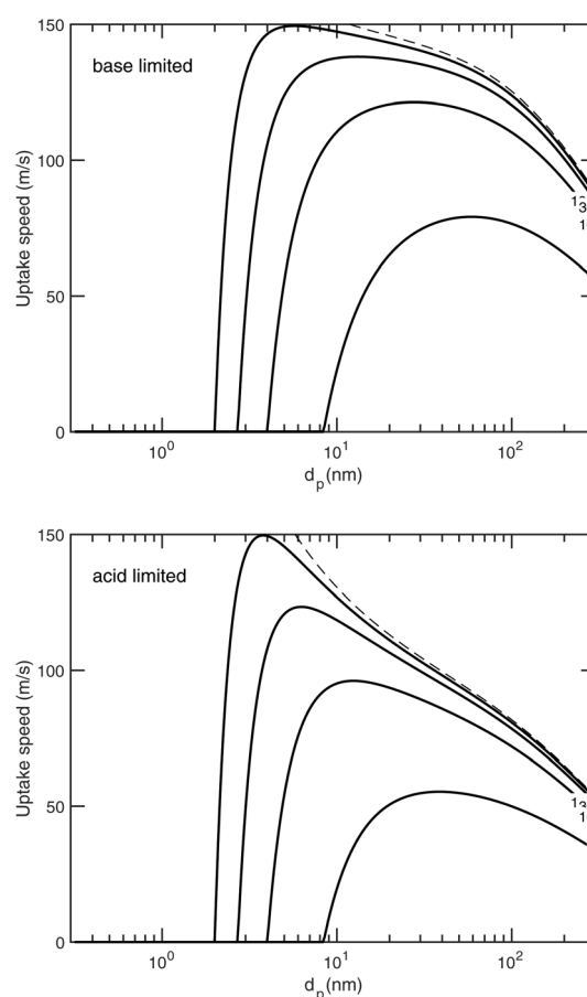
Fig. 17 Uptake speed ( \gamma_{i,p} S_{i,p}^{-1} , black curves) vs. the diameter for flat-surface saturation ratios S^{\circ} = \{3, 10, 30, 100\} and d_{k10} = 2 \text{ nm} . The S^{\circ} = \infty limit is shown as a dashed curve. (Top) Base-limited ( \text{NH}_3 ) limited uptake assuming no van der Waals enhancement ( A = 0 \text{ joule} ). (Bottom) Acid-limited ( \text{HONO}_2 ) uptake with significant van der Waals enhancement ( A = 6 \times 10^{-20} \text{ joule} ). The collision speed (and thus growth rates) increases rapidly after activation, reaches a maximum and then declines again. The maximum is especially sharp when the van der Waals enhancement is large ( i.e. for acid limited conditions in the lower panel).
