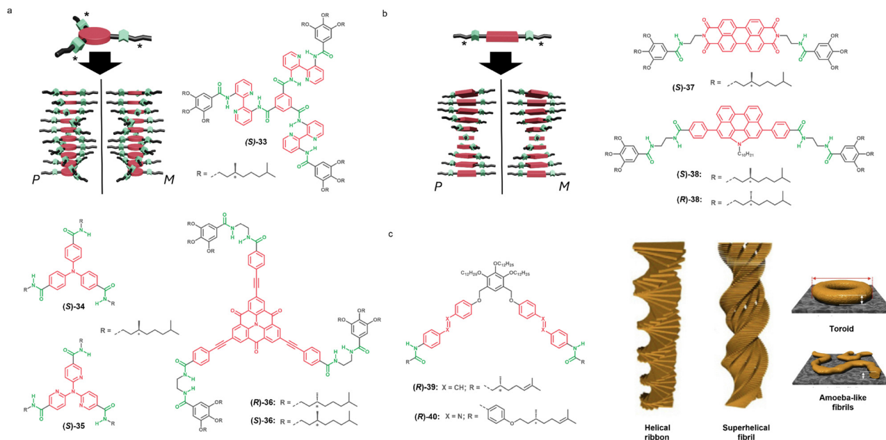
Fig. 12 (a) Schematic representation of the asymmetry transfer in C_3 -symmetry scaffolds upon aggregation by point chirality and BTA ( (S) -33, triarylamines ( (S) -34 and ( (S) -35 and N-heterotriangulenes ( (S) -36 and ( (R) -36 chemical structures. (b) Schematic representation of C_2 -symmetry monomer chiral self-assembly and chemical structure for chiral PBI ( (S) -37 and chiral N-annulated perylenes ( (S) -38 and ( (R) -38 (c) Chemical structures of scissor-shaped monomers endowed with point chirality ( (R) -39 and ( (R) -40 employed by S. Yagai and coworkers and schematic representation of different supramolecular aggregates than can be observed in the supramolecular polymerization process ( (R) -39 depending on the molar fraction of the cross-linked species, namely: helical ribbon, superhelical fibril, toroid and amoeba-like fibrils (reproduced from ref. 196, with permission of Springer Nature, copyright 2015).
