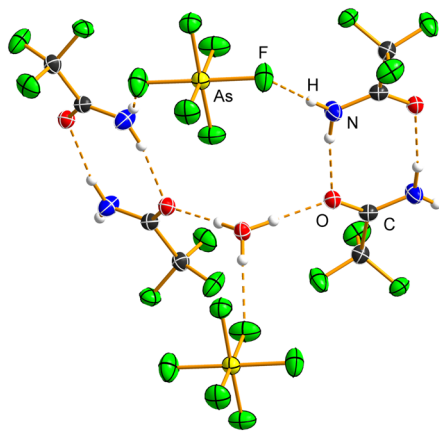
Fig. 5 R 4 4 (14) hydrogen-bonded cluster in the crystal structure of the H 3 O[AsF 6 ] 2 CF 3 CONH 2 salt cocrystal. Hydrogen bonds are shown by dashed orange lines. Displacement ellipsoids are drawn at the 50% probability level, and hydrogen atoms are represented as spheres of arbitrary radius.
