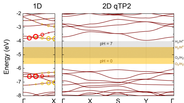
Fig. 15 PBEsol0 band structures of the 1D C_{60} chain and 2D C_{60} networks. The red and yellow circles drawn on the 1D band structures indicate the contributions of the corresponding electron-hole pairs to the two brightest excitons near the band edges. The radii of these circles represent their corresponding oscillator strength. 91
