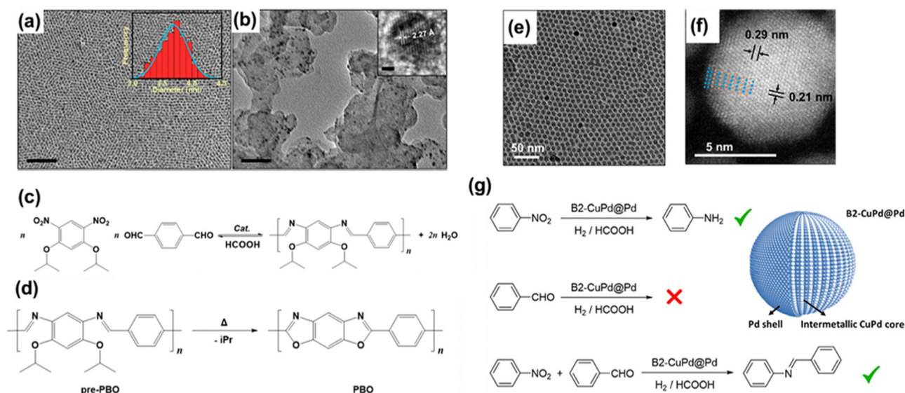
Fig. 8 (a) TEM image of AuPd NPs and (b) AuPd/C. Scale bar: 2 nm, inset 1 nm (c) One-pot synthesis of PBO precursor using diisopropoxy-2,4-dinitrobenzene and terephthalaldehyde. HCOOH is used as a hydrogen source. (d) Transformation of PBO precursor to PBO upon annealing. Reproduced from ref. 192 with permission from American Chemical Society, copyright 2021. (e) TEM images of B2-CuPd NPs with a thin Pd shell. (f) HAADF-STEM image of B2-CuPd. (g) Summary of activity of B2-CuPd with thin Pd shell in catalyzing hydrogenation of nitrobenzene, benzaldehyde, and the Schiff base condensation process. Reproduced from ref. 195 with permission from American Chemical Society, copyright 2024.
