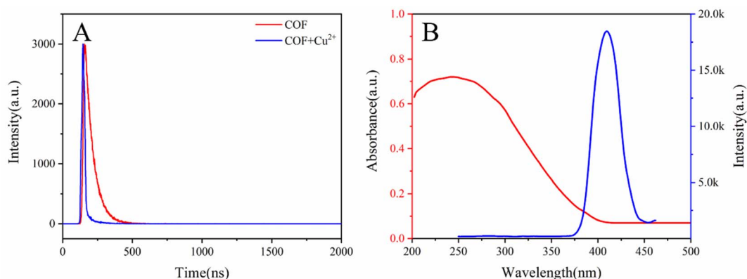
Fig. 6 (A) Fluorescence lifetime (500 nm) of the TPE-Bpy-COF sensor in the absence of \text{Cu}^{2+} /presence of \text{Cu}^{2+} . (B) UV absorption spectra of \text{Cu}^{2+} (red line) and excitation spectrum of the TPE-Bpy-COF sensor (blue line).
