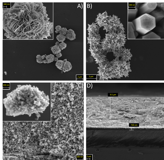
Fig. 2 FESEM images for different ZnO morphologies, namely (A) DRs, (B) MPs, and (C) NPs. (D) Cross-section image of a NPs-based photoanode.
