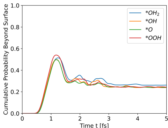
Fig. 5 Cumulative probability beyond the surface, Ni doped hematite. Hole propagation.
