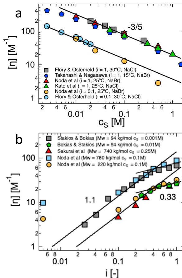
Fig. 22 (a) Dependence of intrinsic viscosity of polyacrylic acid on added salt concentration for N \approx 8170 (see text) for 10% ionisation ( i = 0.1 ) and full ionisation ( i = 1 ). Power-law of -3/5 is the scaling prediction. (b) Intrinsic viscosity vs. degree of neutralisation i . Exponents are best fit values. Data are from ref. 195, 537 and 540–543. Results reported by Bokias and Stakios 542 were obtained by isoionic dilution.
