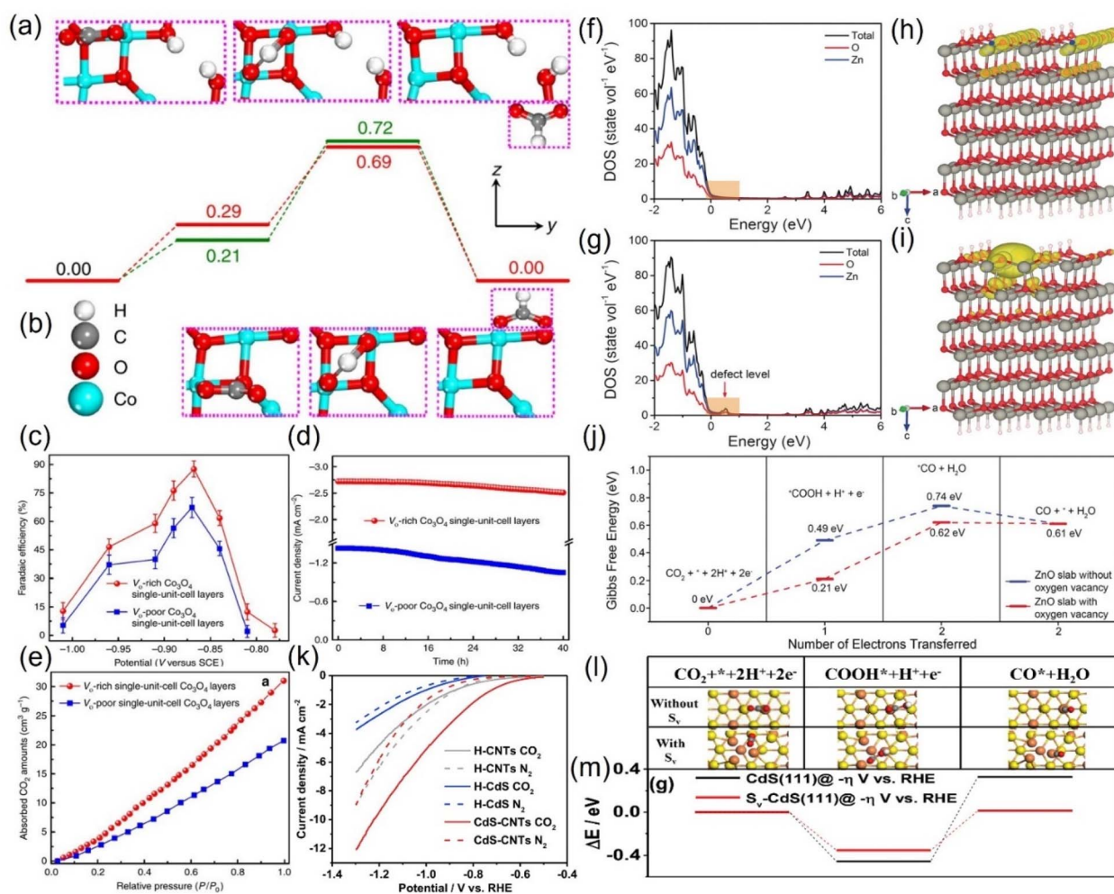
Fig. 8 Gibbs free energy diagrams of (a) V_{O} -rich and (b) V_{O} -poor single-unit-cell Co_3O_4 layers. (c) FE_{HCOOH} at different applied potentials. (d) Chronoamperometry tests and (e) CO_2 adsorption isotherms of VO -rich/poor single-unit-cell Co_3O_4 layers. (f and g) DOS. (h and i) Charge density distribution and (j) Gibbs free energy diagrams of (f and h) ZnO slab and (g and i) ZnO slab with oxygen vacancy. (k) LSV curves. (l) Models of different intermediates and (m) DFT calculation results of corresponding intermediates during CO_2RR on CdS without/with S-vacancy ( S_v ). (a–e) Reproduced with permission. 104 Copyright 2017, Springer Nature. (f–j) Reproduced with permission. 105 Copyright 2018, John Wiley and Sons Ltd. (k–m) Reproduced with permission. 107 Copyright 2020, Royal Society of Chemistry.
