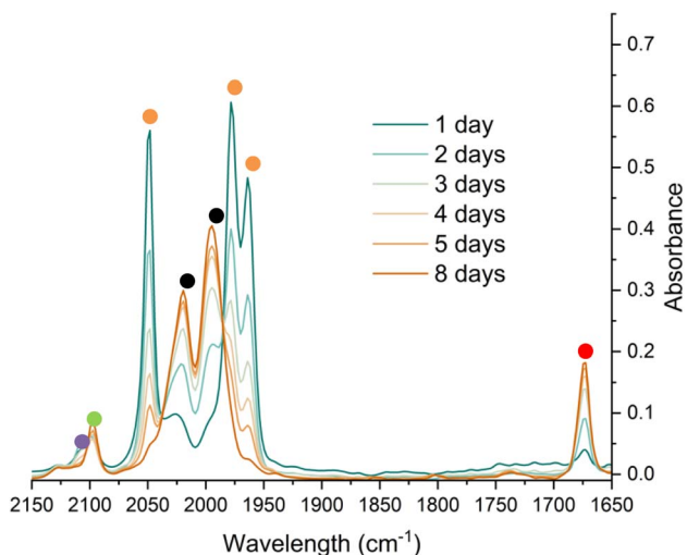
Fig. 7 IR spectroscopic monitoring using a Harrick cell of the reaction of 4^{Mes} under an atmosphere of CO in toluene over 8 days. Orange circles highlight the signals for 4^{Mes} , red circles highlight the signals for 2^{Mes} . Black circles highlight the signals for Fe(CO)_5 . The green circle highlights the signal for 8 . The purple circle highlights a signal attributed to a proposed Fe–ketenyl complex, 9 (see Fig. 8 for proposed structure). See ESI† for a zoom in of the region between 2150–2075 cm^{-1} .
