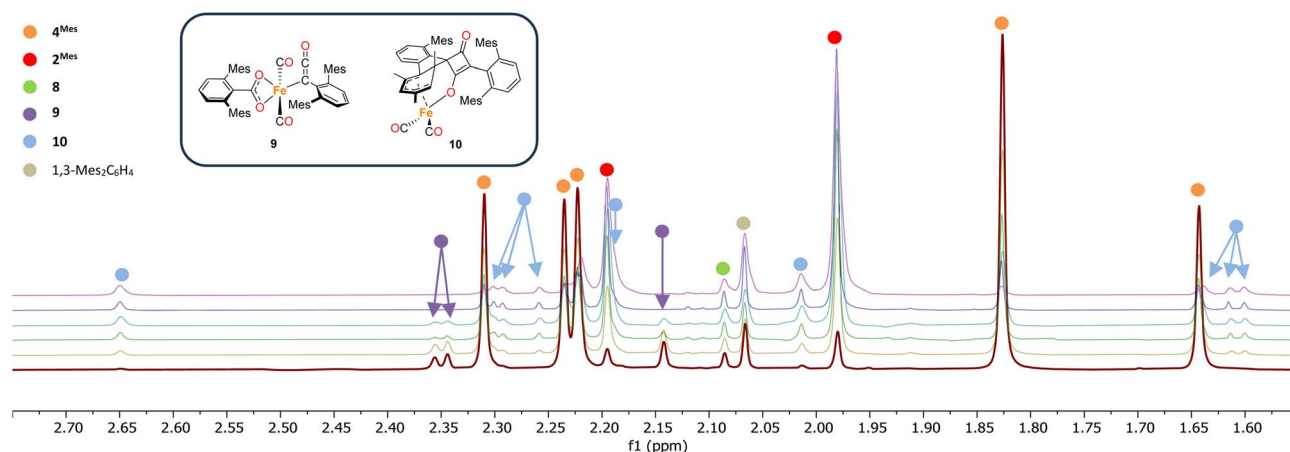
Fig. 8 ^1H NMR spectra of the reaction of 4^{Mes} with CO in C_6H_6 . Spectra collected on after reacting for 1 (red), 2 (yellow), 3 (green), 4 (light blue), 5 (dark blue) and 8 (purple) days. Time increases from bottom to top. Corresponding para methyl signals for 8 and 1,3-Mes _2 C _6 H _4 overlap with other signals and are not shown. See the ESI for full spectrum (Fig. S56)† and further details on how the data was collected. Inset, structures of proposed Fe–ketenyl intermediate 9 and cyclobutenone byproduct 10 .
