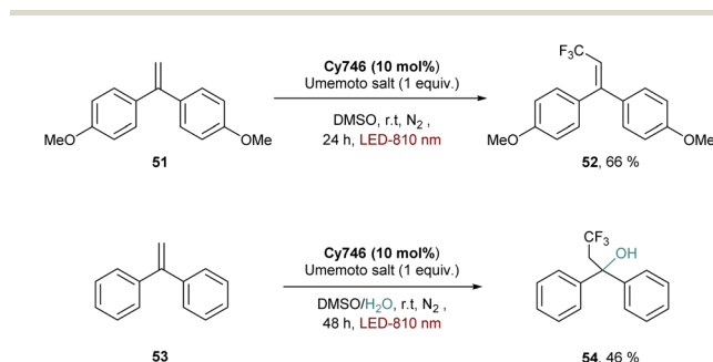
Scheme 14 Reduction of the Umemoto salt with Cy746 .
