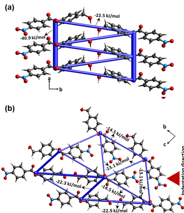
Fig. 7 Energy framework calculations were performed for crystal 4 , along the a -axis for \pi -stacked units and (b) in the bc -plane.
