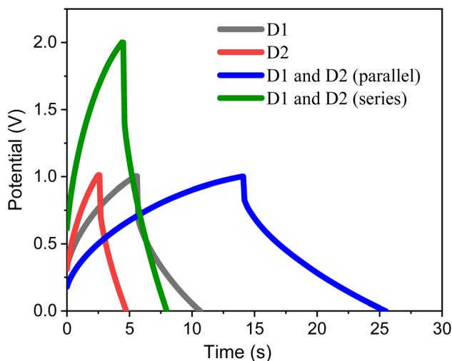
Fig. 8 GCD curves recorded for two different symmetric coin cell supercapacitor devices (D1 and D2) connected in parallel and series at a current density of 1 \text{ mA cm}^{-2} .
