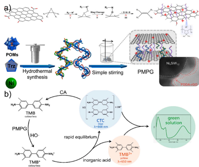
Fig. 4 Applications of the Ni 4 SiW 12 /PDDA-rGO in the detection of CA. (a) Schematic illustration of synthesizing Ni 4 SiW 12 /PDDA-rGO. (b) Schematic illustration of detecting CA using Ni 4 SiW 12 /PDDA-rGO. 29 Copyright 2020, Elsevier.
