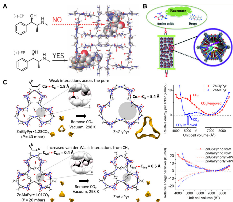
Fig. 7 (A) Mechanism of \text{Cu}(\text{GHG}) for chiral recognition and discrimination. Reproduced with permission from ref. 82. Copyright 2017 American Chemical Society. (B) Illustration of lysozyme @ COF 1 based CSPs for chiral separation. Reproduced with permission from ref. 83. Copyright 2018 Wiley. (C) Mechanism of \text{ZnXPyr} \text{CO}_2 removal and calculated E-V curves. Reproduced with permission from ref. 84.
