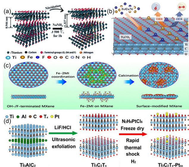
Fig. 4 (a) Synthesis procedures for the N-Ti 2 CT x nanosheets and their dispersion. 46 Copyright 2018, Royal Society of Chemistry. (b) Mechanisms for the formation of Fe/Co/Ni-DACs based on Ti 2 CO 2 and for the electrocatalytic reactions in aqueous electrolytes. 52 Copyright 2021, Wiley. (c) Schematic illustration for the preparation procedure of the surface-tuned MXene/TiFeO x nanosheets. 51 Copyright 2020, American Chemical Society. (d) Schematic illustration of constructing Pt single atoms on monolayer Ti 3 C 2 T x . 53 Copyright 2022, American Chemical Society.
