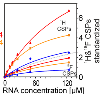
Fig. 8 Estimated affinity plots of chemical shift perturbation against RNA concentration by stepwise titration of 5_SL2 + 3 ext and 5_SL4 to DRTL A04 and DRTL B04 via 1 H and 19 F NMR over various RNA concentrations at a fixed compound concentration. CSP values were standardised with the observed spectral dispersion in Hertz of 1 H or 19 F 1D experiments, respectively. The grey dotted line indicates the border of the ranges of values between 1 H and 19 F CSPs induced by ligand binding.
