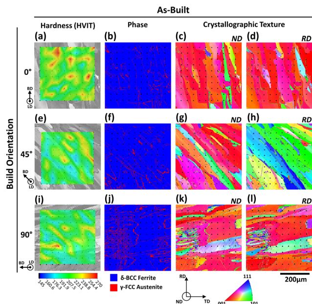
Fig. 13 Instrumented indentation mapping of the as-built samples with corresponding phase, and crystallographic texture maps in the ND and RD, taken in the; (a)–(d) 0^\circ , (e)–(h) 45^\circ and (i)–(l) 90^\circ build orientations.
